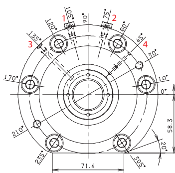
Clamping Head 110
