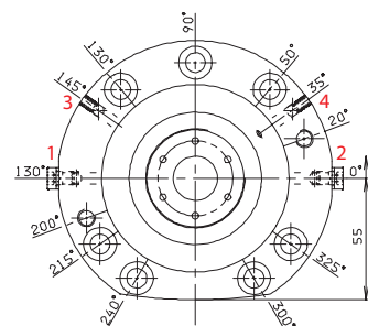
Clamping Head 125
