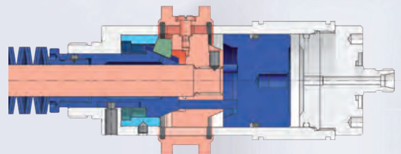
Clamped position
